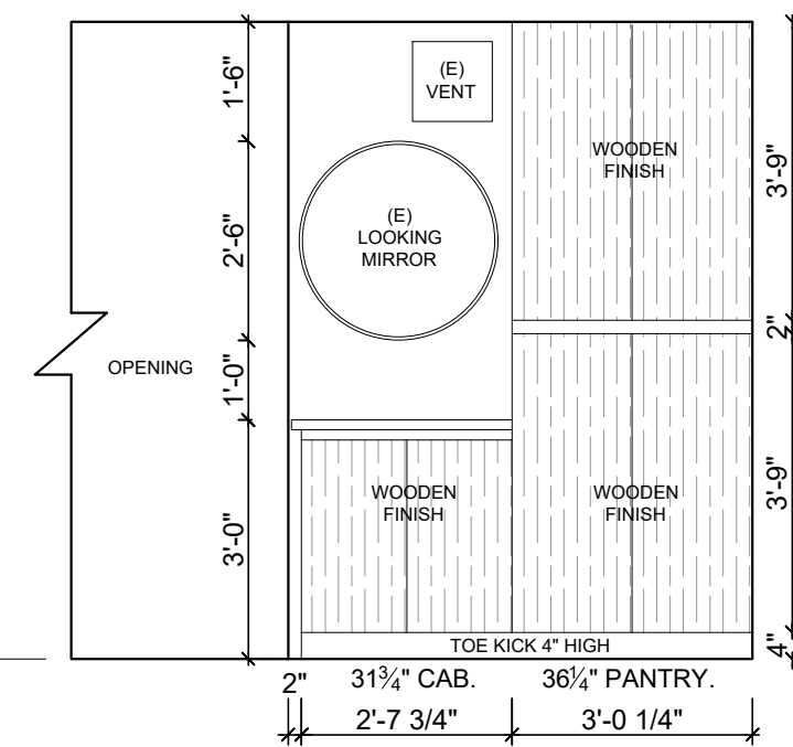
ELEVATION-C
