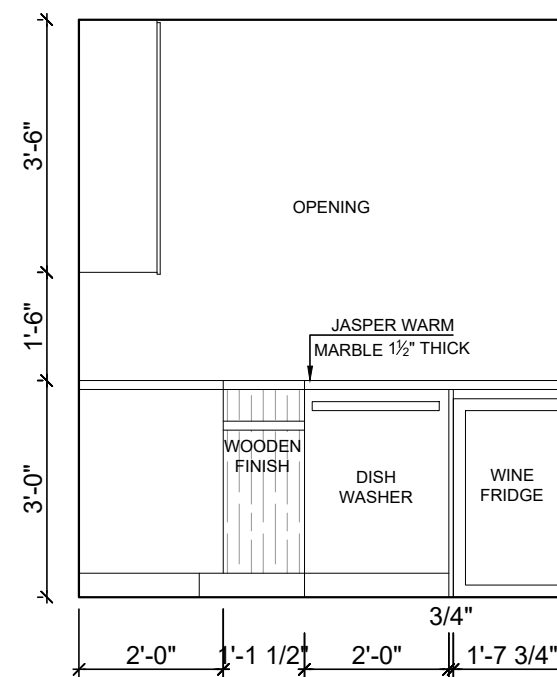
ELEVATION-B
